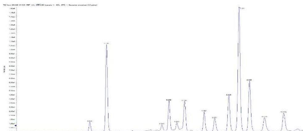
Chromatographic Separation
